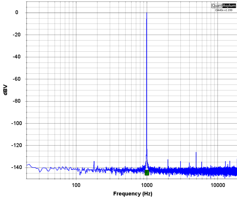
Figure 1: Screen Shot of the QA403 Loopback Measurement
