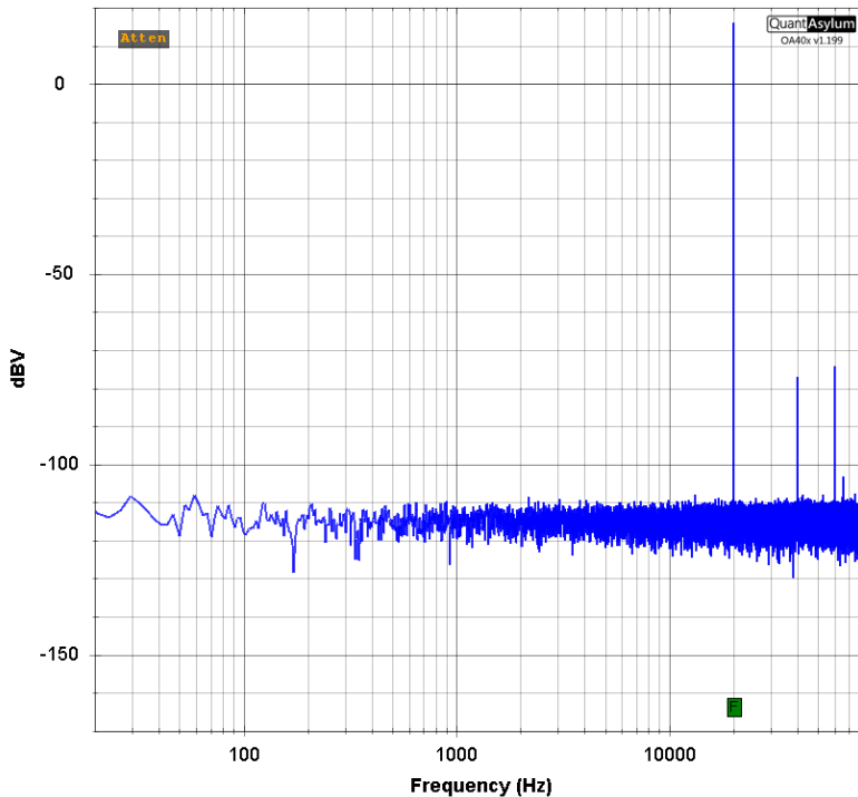
Figure 11: THD-20 Spectrum at 5 Watts
