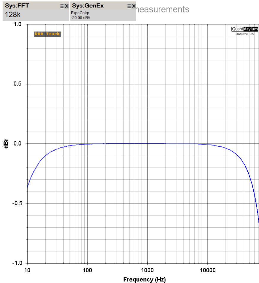
Figure 3: Frequency Response Measurement 10 Hz to 80 kHz
