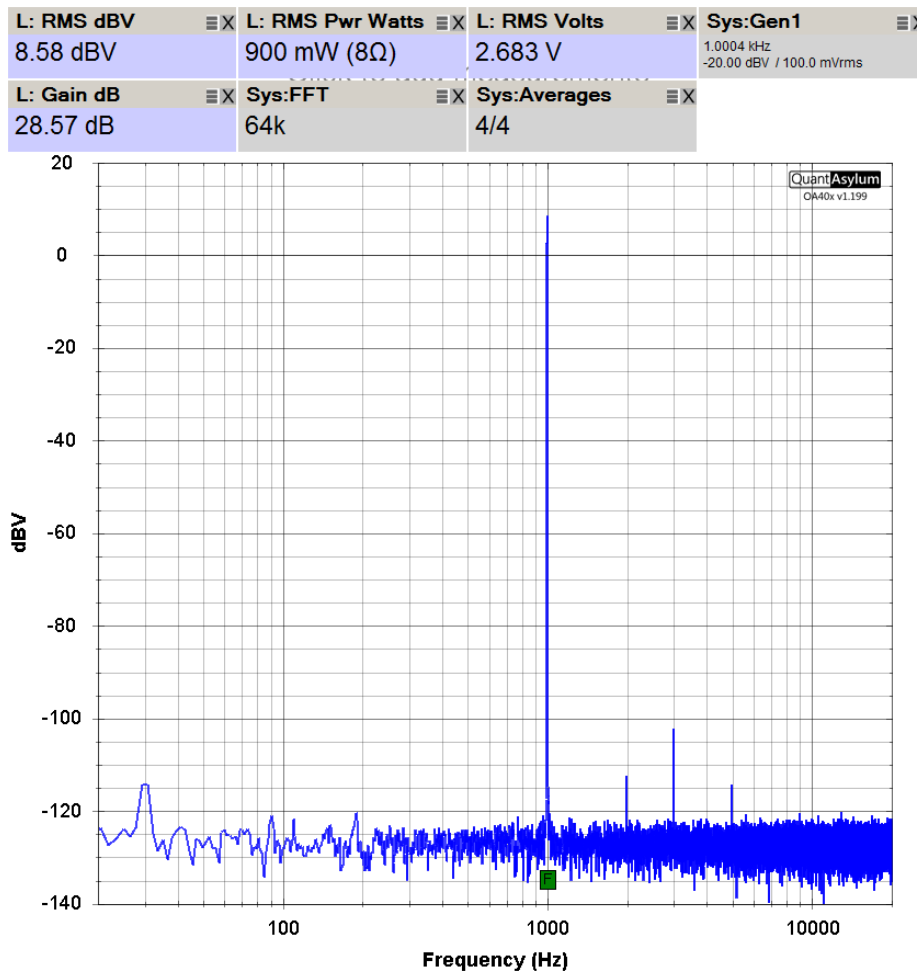
Figure 2: Screen Shot of the Amplifier Gain Measurement
