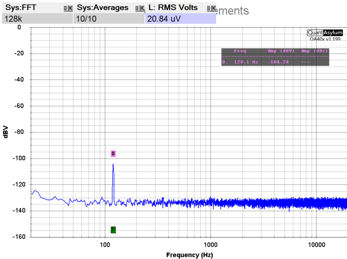
Figure 4: Amplifier Un-weighted Output Noise
