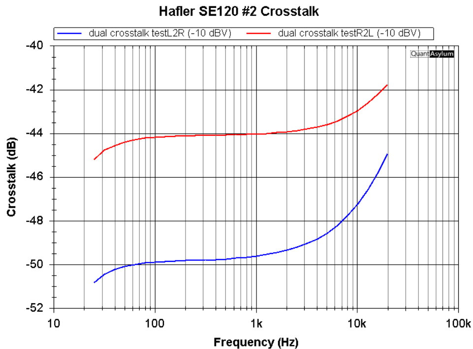
Figure 35: Crosstalk of a Hafler SE120 Stereo Amplifier
