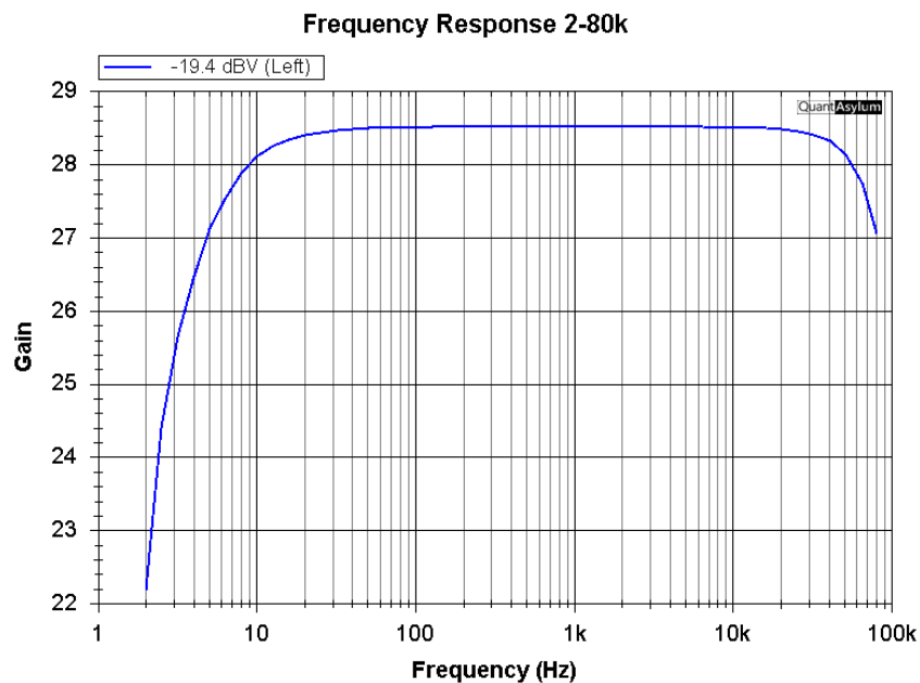
Figure 31: Frequency Response 2 Hz to 80 kHz
