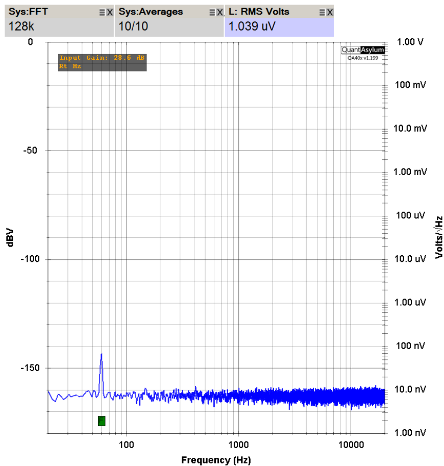
Figure 8: Input-referred Noise Density
